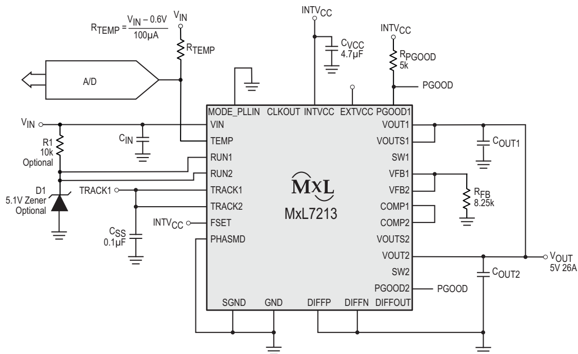
Figure 32: 2-Phase, 5V at 26A with Temperature Monitoring
