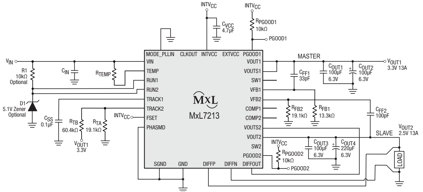
Figure 28: Example of Output Tracking Application Circuit
