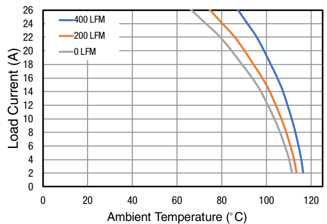
Figure 39: Power Derating, V_{IN} = 12V, V_{OUT} = 2.5V
