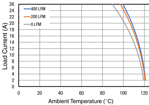
Figure 36: Power Derating, V_{IN} = 12V, V_{OUT} = 1.0V
