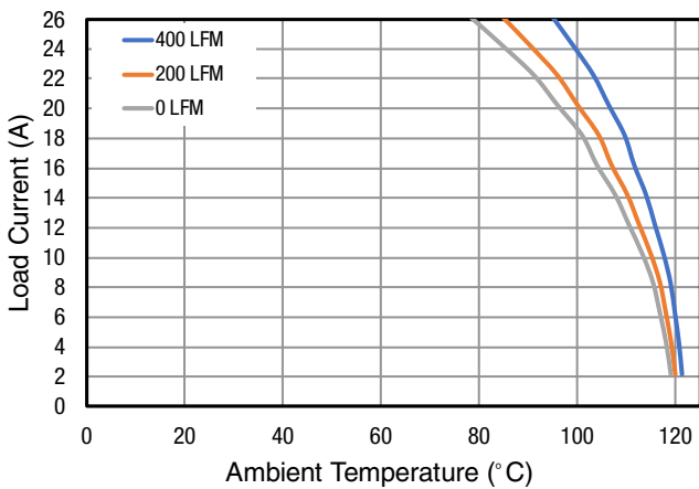
Figure 38: Power Derating, V_{IN} = 5V, V_{OUT} = 2.5V
