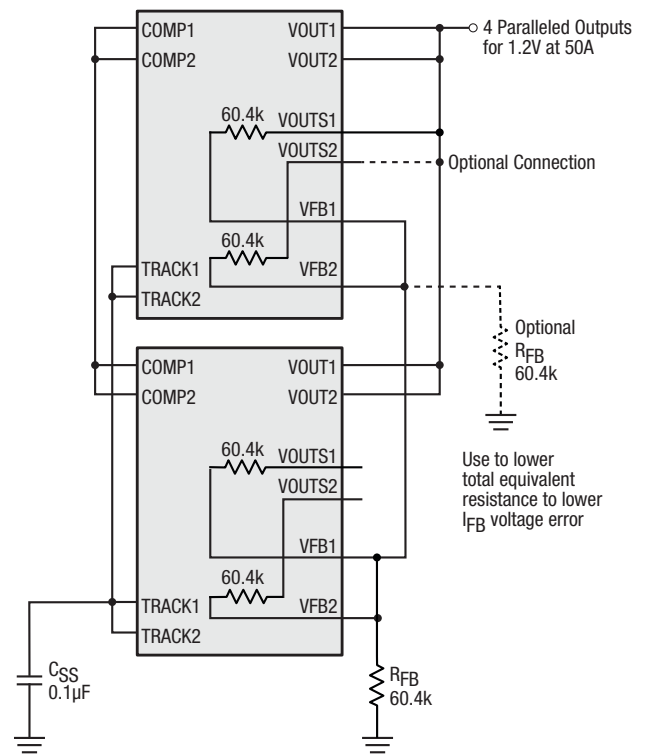
Figure 23: 4-Phase Parallel Configuration
