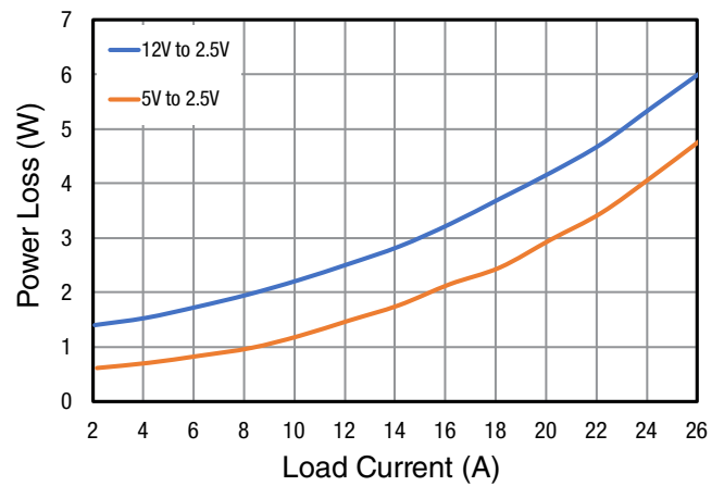
Figure 37: Power Loss, V_{OUT} = 2.5V
