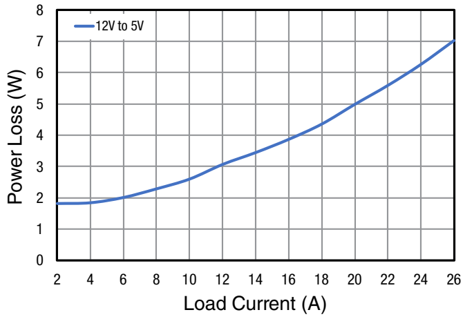
Figure 40: Power Loss, V_{OUT} = 5V
