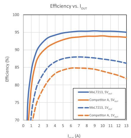
Figure 2: Efficiency Advantage vs. Competition
