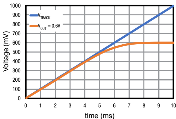
Figure 27: V_{OUT} and V_{TRACK} versus Time
