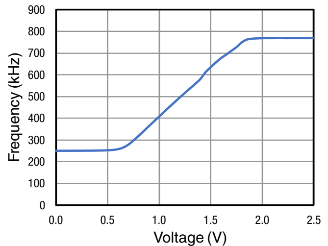
Figure 26: Operating Frequency vs. FSET Pin Voltage
