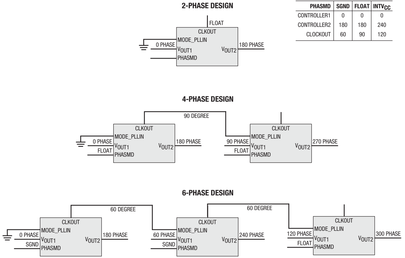
Figure 24: Examples of 2-Phase, 4-Phase and 6-Phase Operation with PHASMD Table
