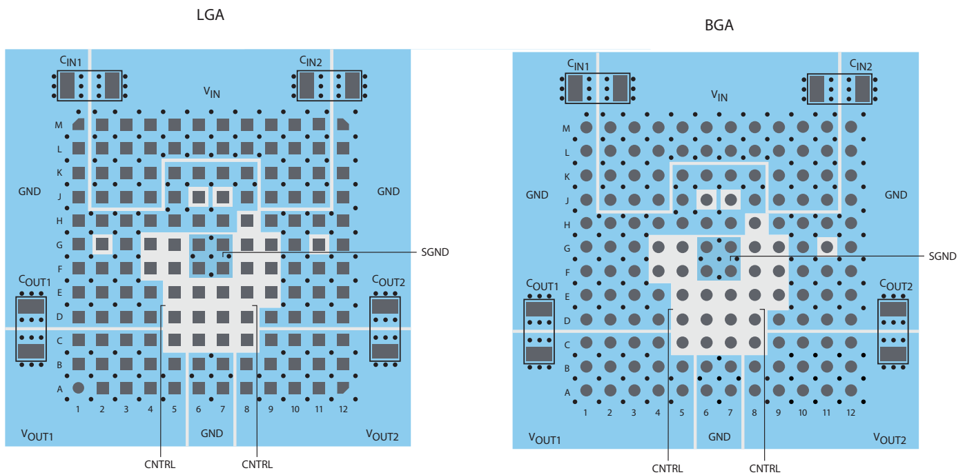
Figure 42: Recommended PCB Layout
