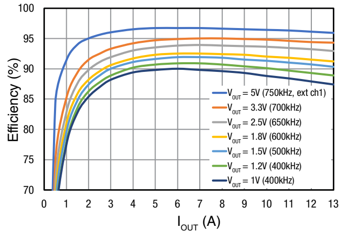
Figure 5: Efficiency: Single Phase, V_{IN} = 8V
