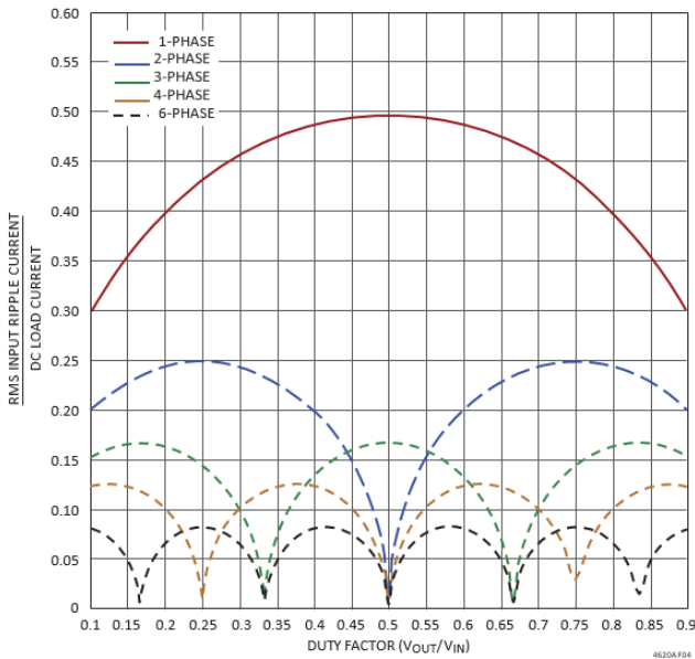
Figure 25: Normalized Input RMS Ripple Current vs. Duty Cycle, One to Six Phases
