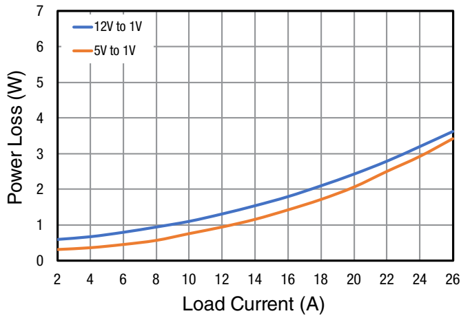
Figure 34: Power Loss, V_{OUT} = 1.0V
