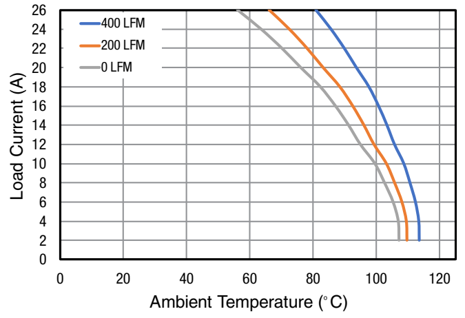
Figure 41: Power Derating, V_{IN} = 12V , V_{OUT} = 5V
