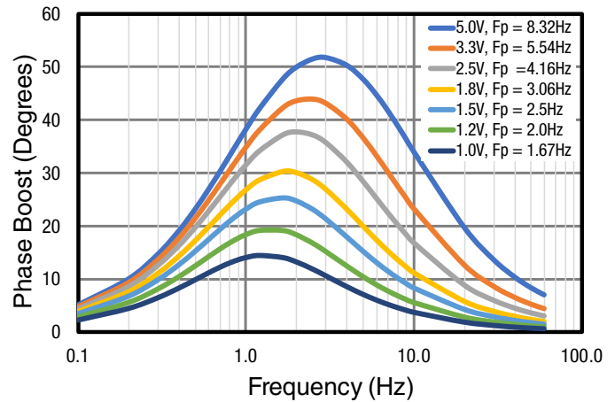
Figure 30: C FF Phase Boost vs. Frequency Fzero Normalized to 1
