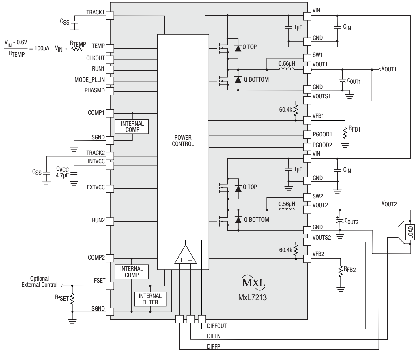
Figure 21: Functional Block Diagram
