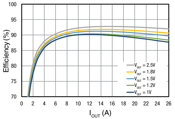
Figure 7: Efficiency: Dual Phase, V_{IN} = 12V
