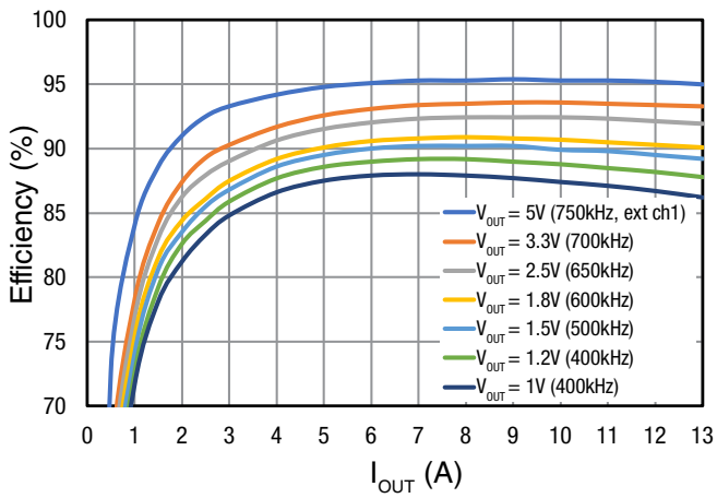
Figure 6: Efficiency: Single Phase, V_{IN} = 12V
