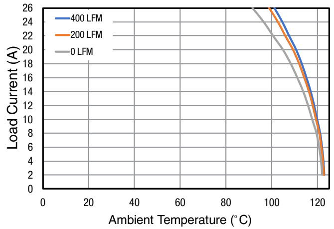
Figure 35: Power Derating, V_{IN} = 5V, V_{OUT} = 1.0V
