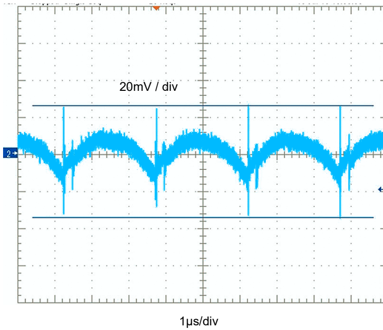
Figure 20: MxL7213 Output Voltage Noise (BW 500MHz)
