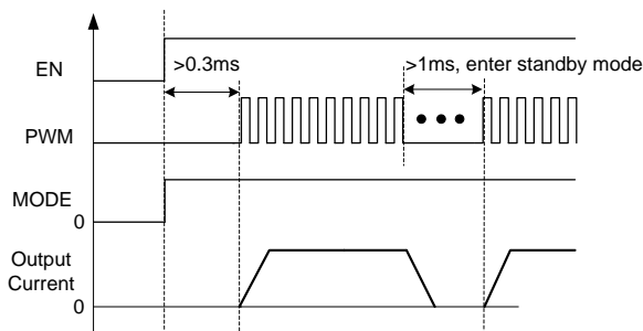
Figure 2: Positive Output Current Mode
