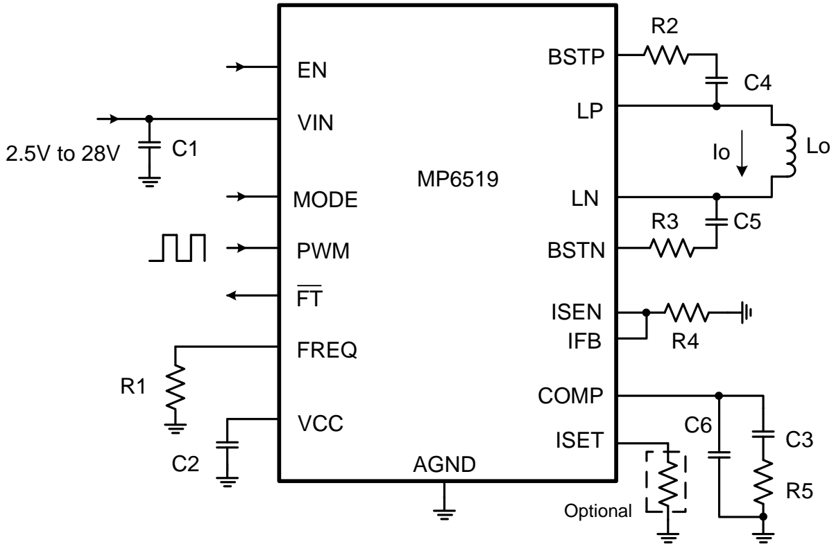
Figure 6: Typical Application
