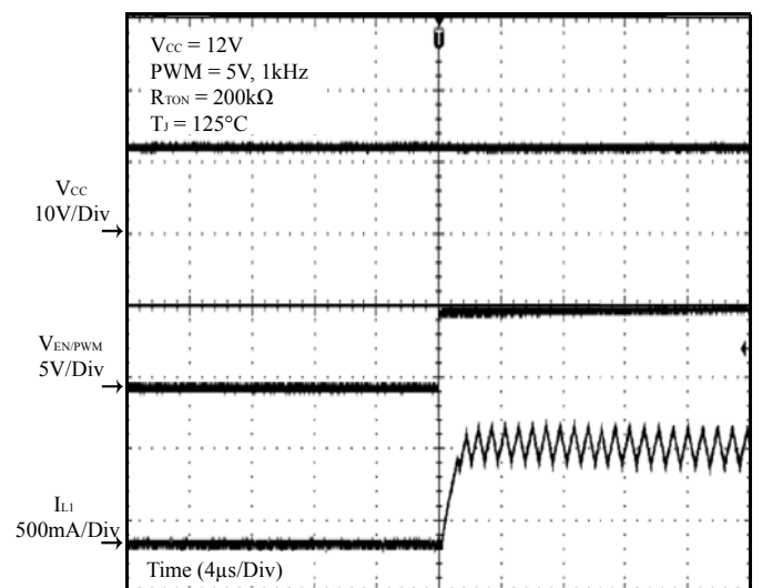
Figure 25 PWM On
