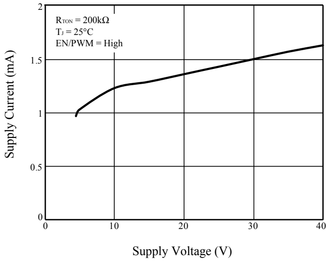
Figure 2 I_{CC} vs. V_{CC}
