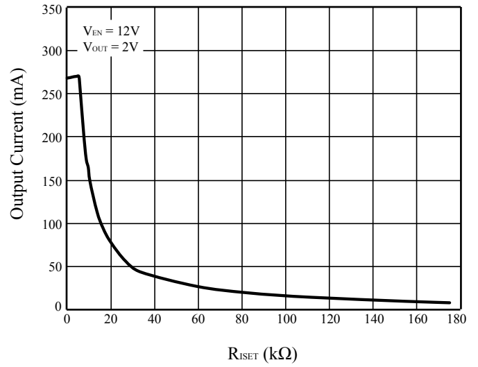
Figure 11 Output Current vs. R_{SET}
