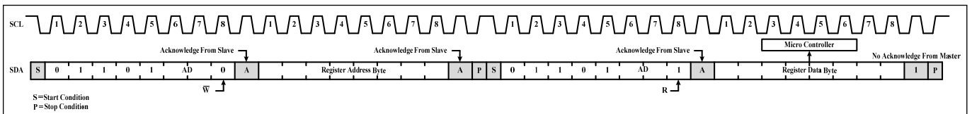
Figure 6 Reading from IS31FL3237
