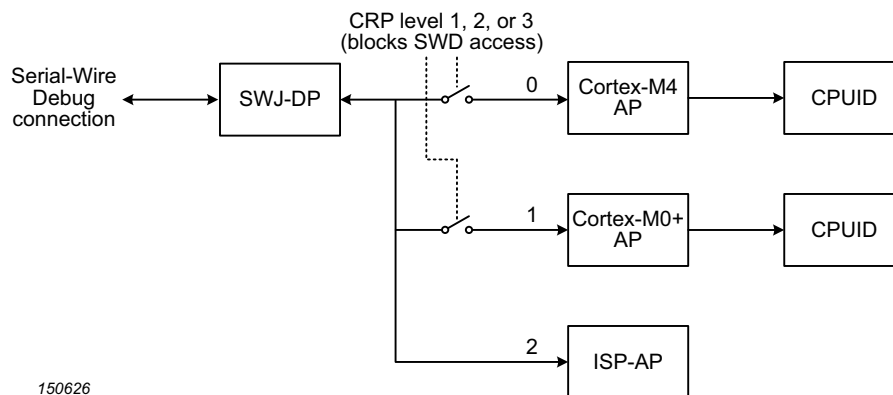
Fig 96. Serial Wire Debug internal connections
