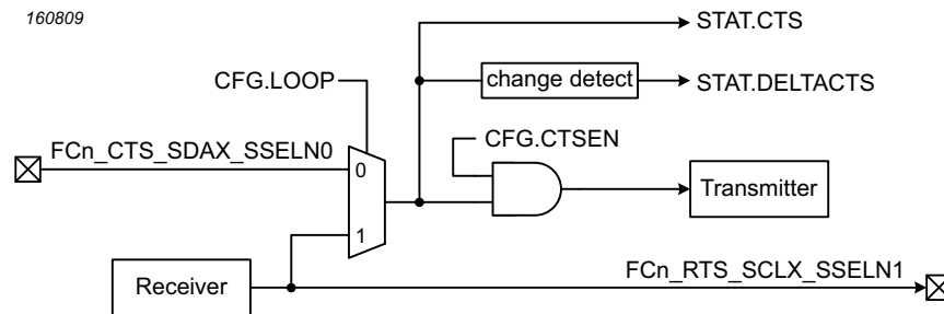
Fig 57. Hardware flow control using RTS and CTS
