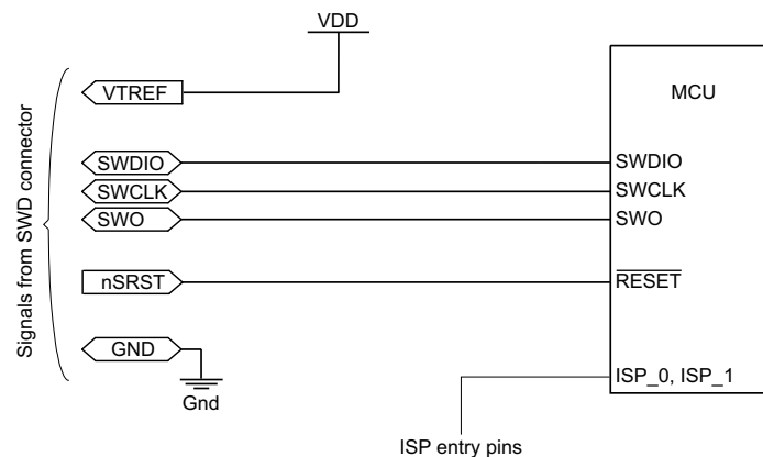
Fig 95. Connecting the SWD pins to a standard SWD connector
