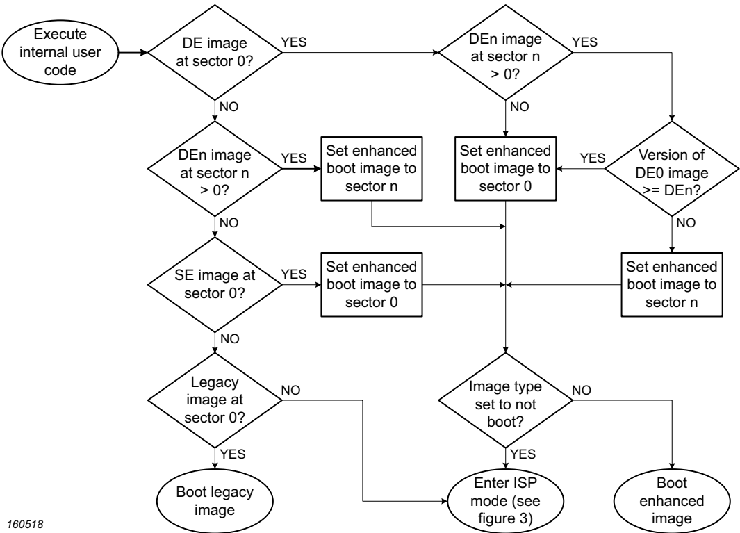
Fig 5. Simplified boot flow, figure 2
