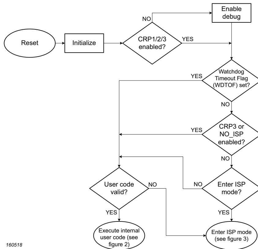
Fig 4. Simplified boot flow, figure 1
