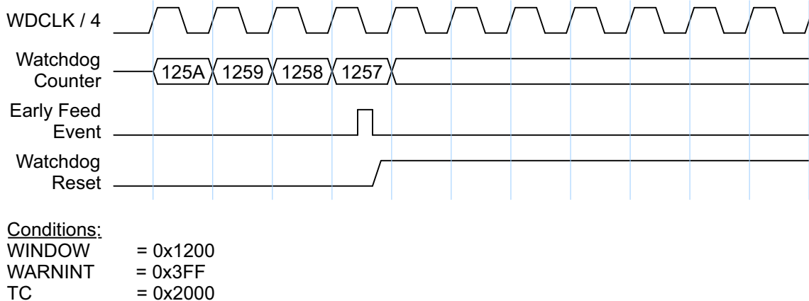
Fig 43. Early watchdog feed with windowed mode enabled
