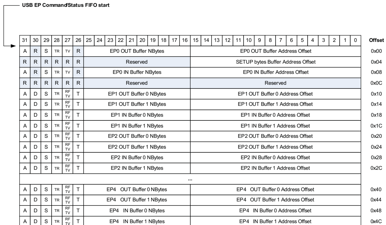
Fig 52. Endpoint command/status list (see also Table 379 )
