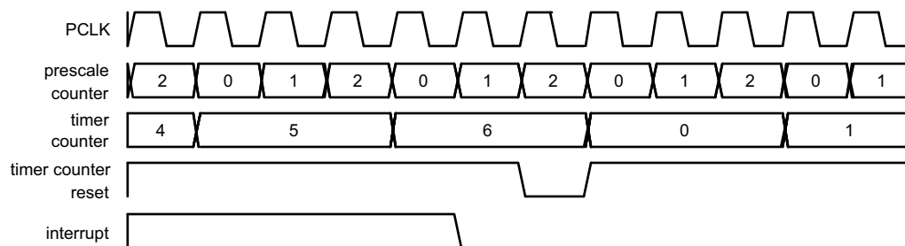
Fig 38. A timer cycle in which PR=2, MRx=6, and both interrupt and reset on match are enabled
