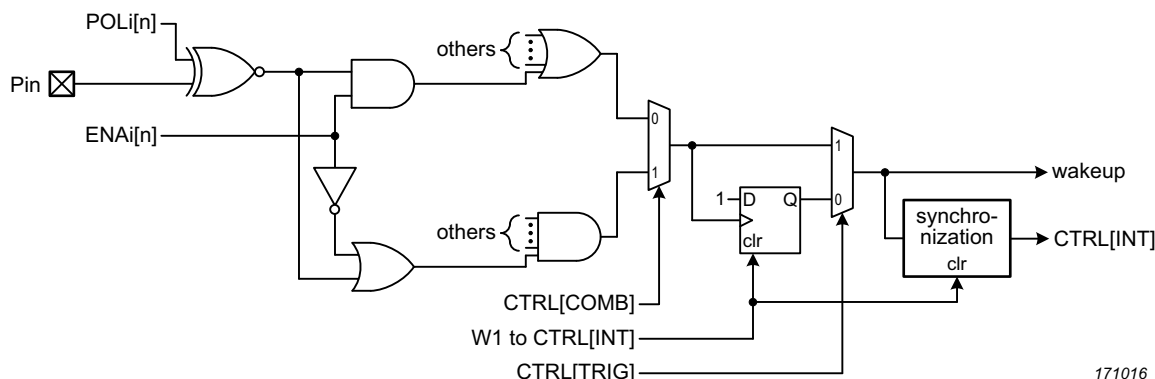
Fig 23. Group GPIO interrupt block diagram
