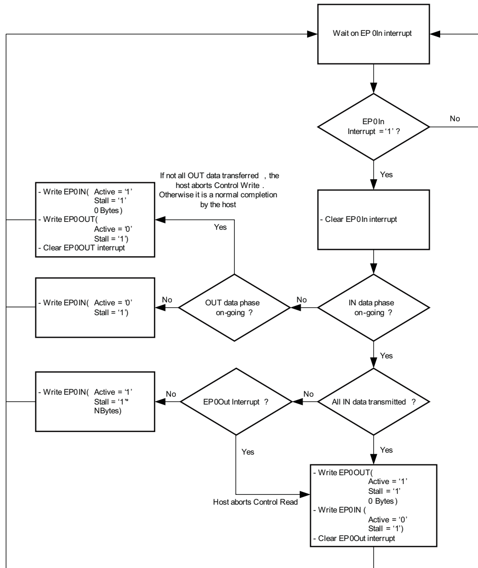
Fig 54. Flowchart of control endpoint 0 - IN direction
