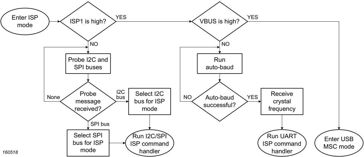
Fig 6. Simplified boot flow, figure 3
