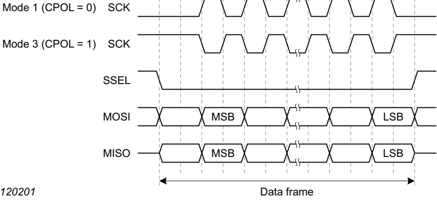
Fig 59. Basic SPI operating modes
