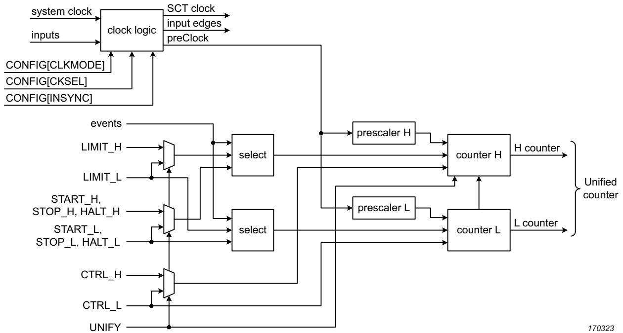
Fig 29. SCTimer/PWM counter and select logic
