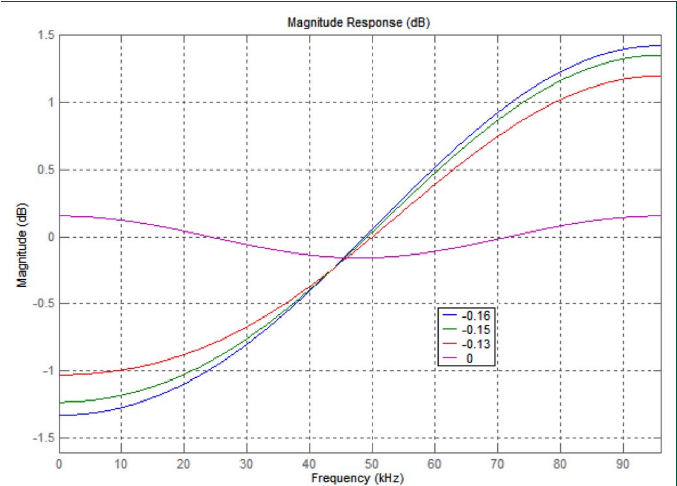
Fig 84. Pre-emphasis filter quantized response at 96 kHz
