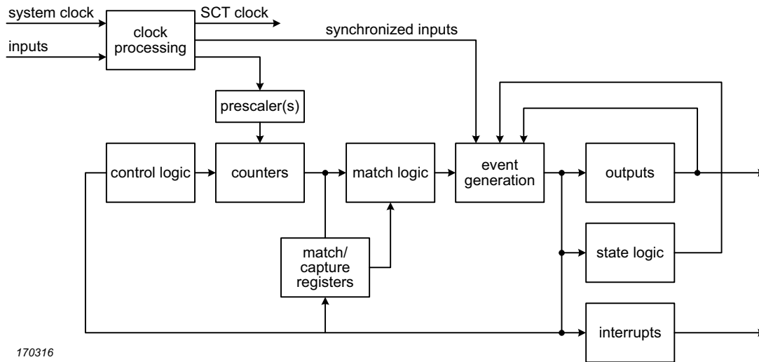
Fig 28. SCTimer/PWM block diagram
