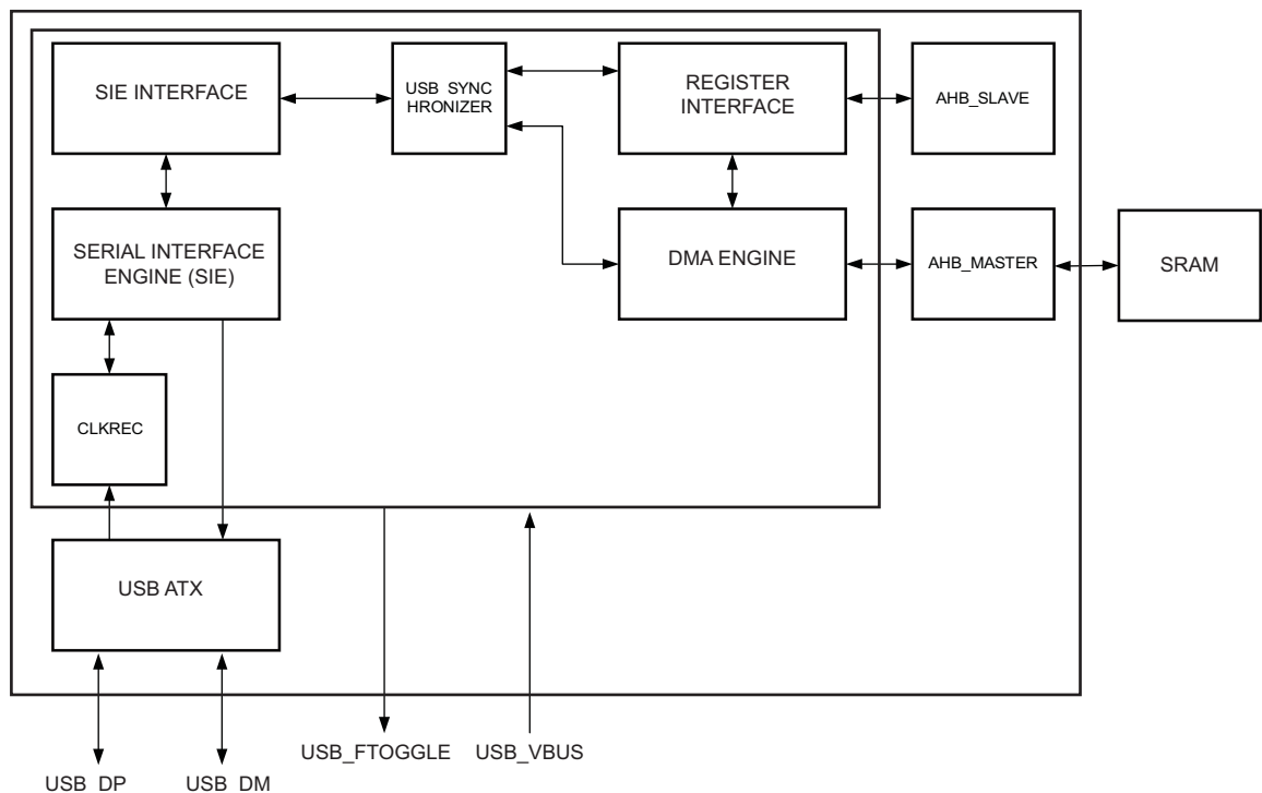
Fig 50. USB block diagram
