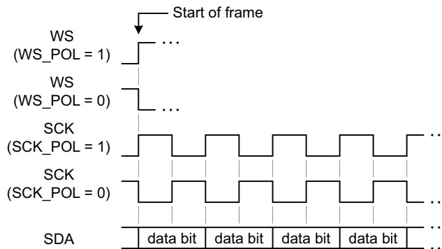
Fig 77. Data at the start of a frame, shown with both SCK and WS polarities
