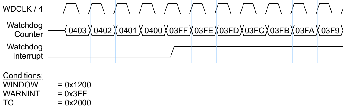
Fig 45. Watchdog warning interrupt
