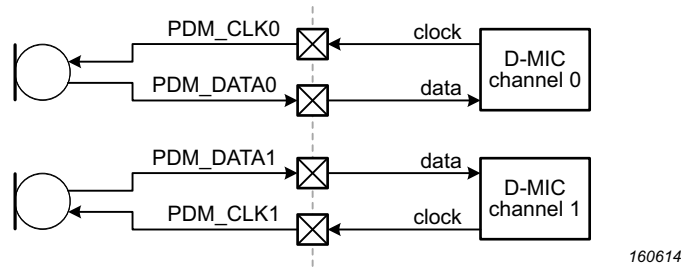
Fig 79. Typical connection to two independent microphones
