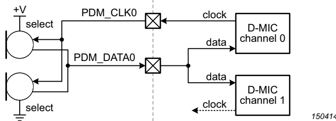
Fig 80. Typical connection to two microphones sharing a data line
