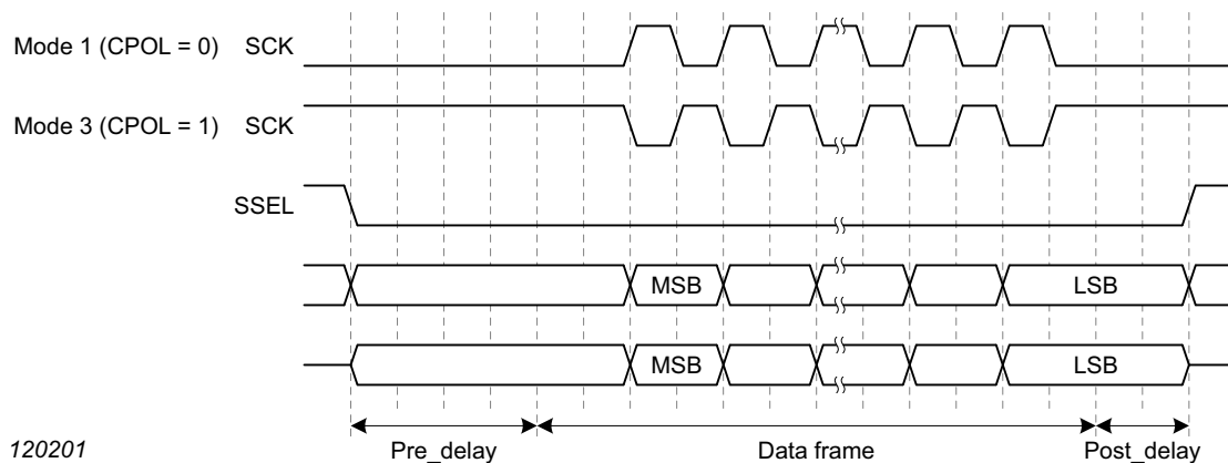
Fig 60. Pre_delay and Post_delay
