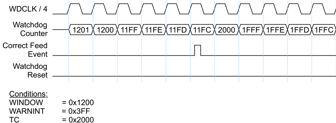
Fig 44. Correct watchdog feed with windowed mode enabled
