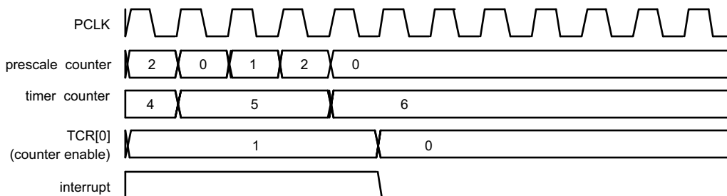
Fig 39. A timer cycle in which PR=2, MRx=6, and both interrupt and stop on match are enabled
