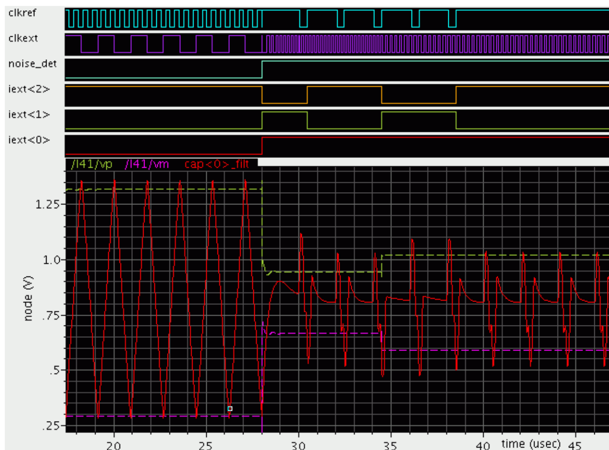
Figure 41-16. TSI noise detection mode waveform
