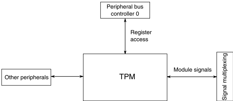
Figure 3-25. TPM configuration
