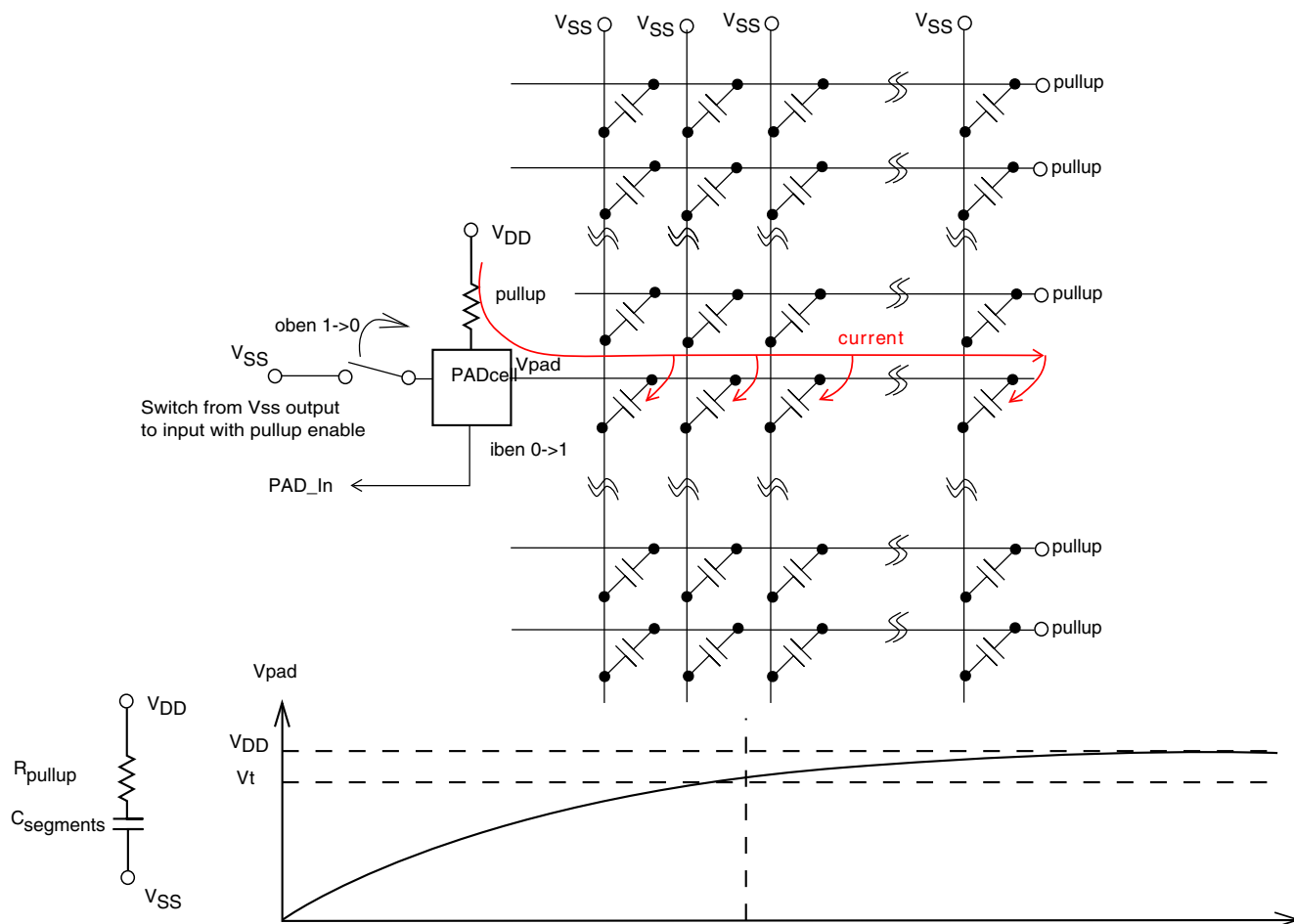
Figure 42-33. Pullup fault detect in connection/segment normal case
