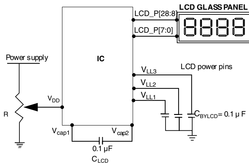
Figure 42-43. Power connections for contrast control
