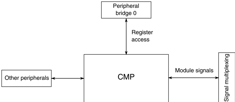
Figure 3-23. CMP configuration
