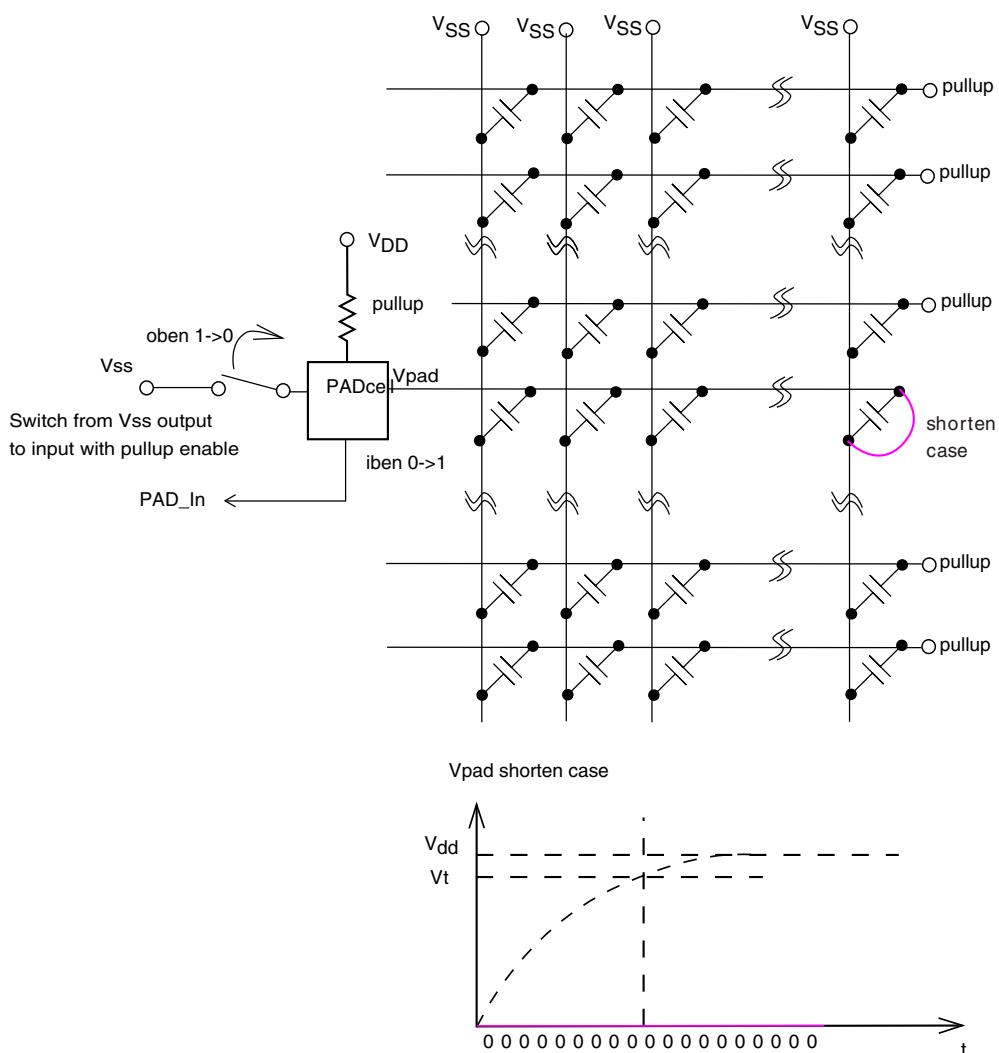
Figure 42-35. Pullup fault detect in connection/segment short case
