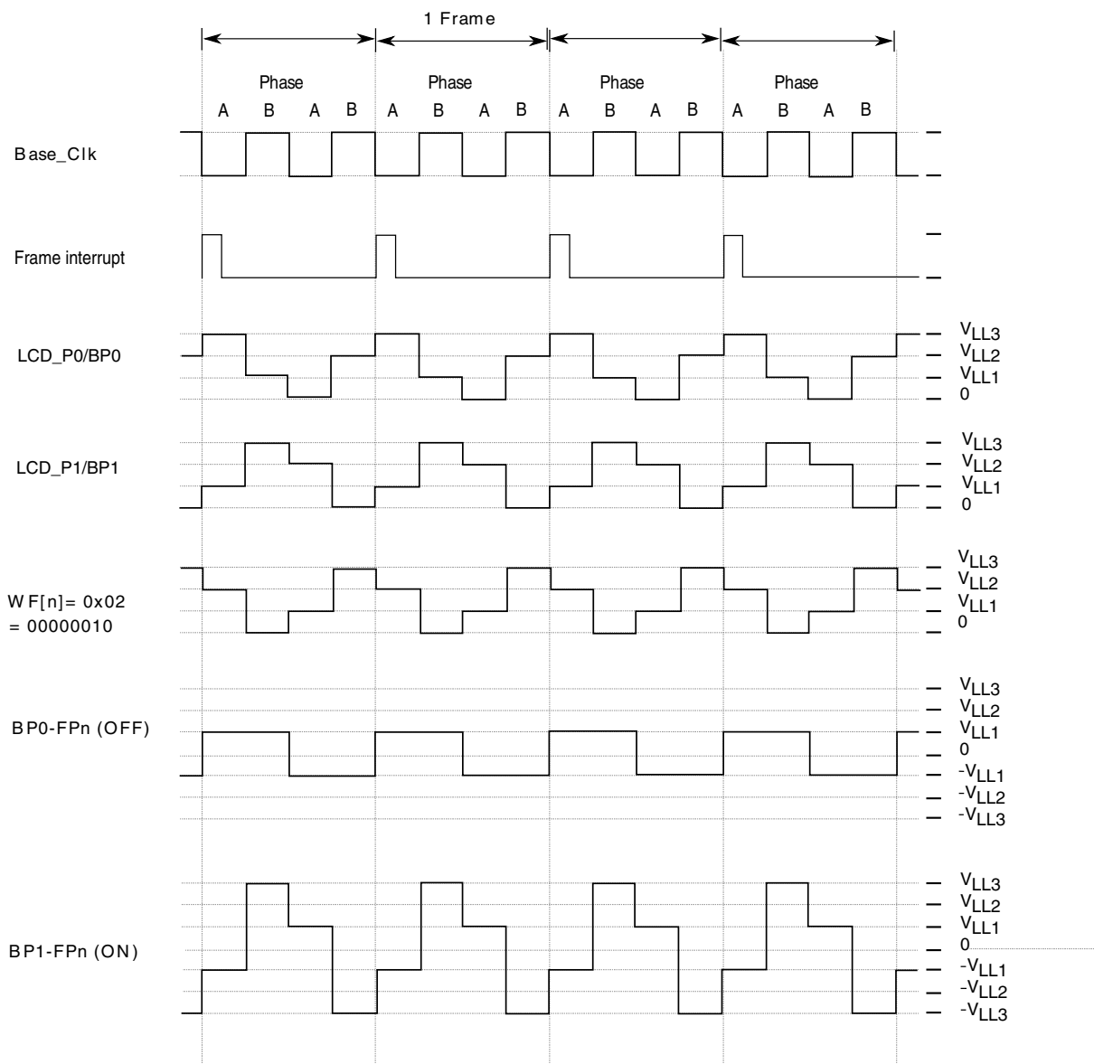
Figure 42-29. 1/2 duty and 1/3 bias (low-power waveform)
