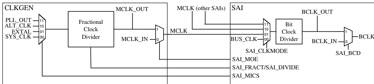
Figure 39-38. SAI master clock generation
